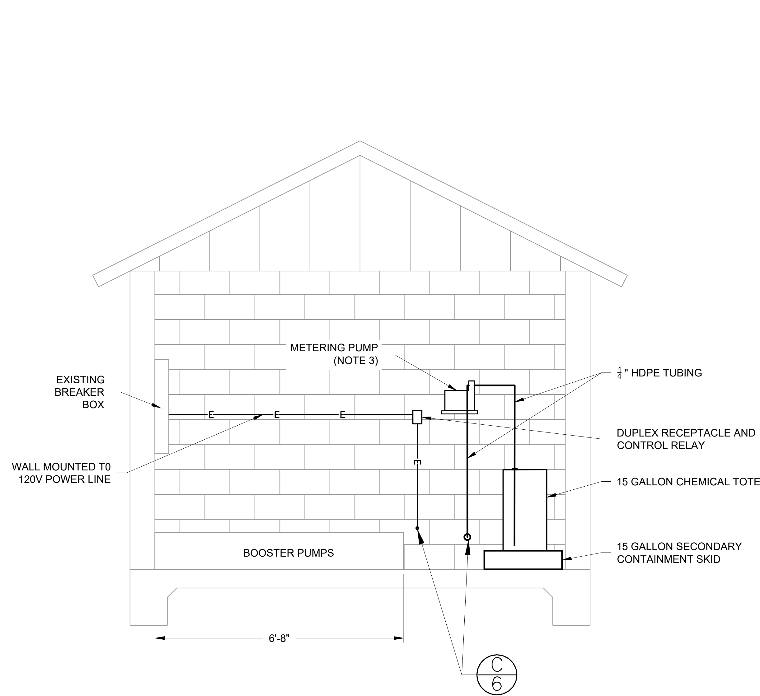
SECTION VIEW
