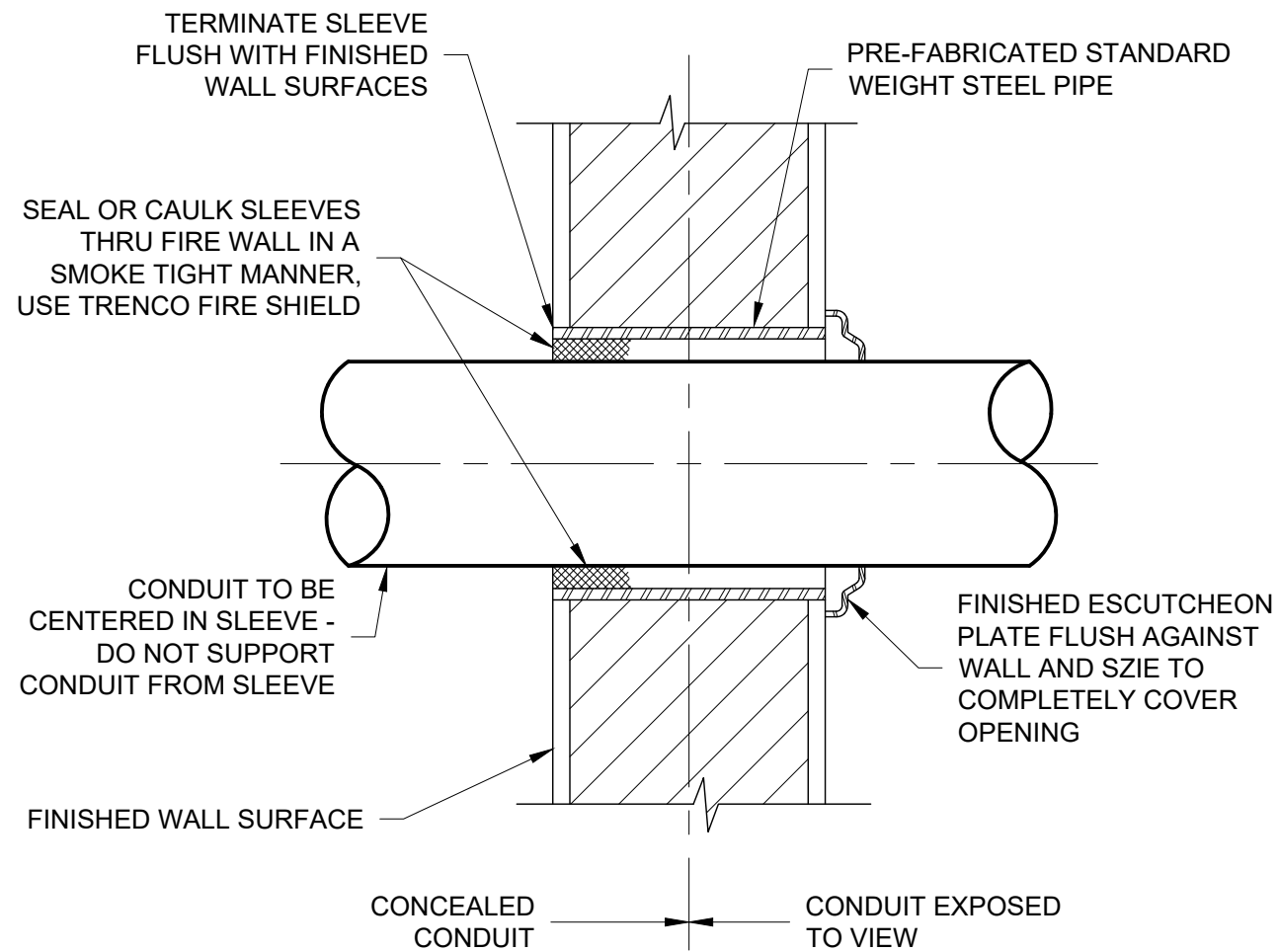
C CONDUIT SLEEVE THROUGH WALLS NOT TO SCALE
