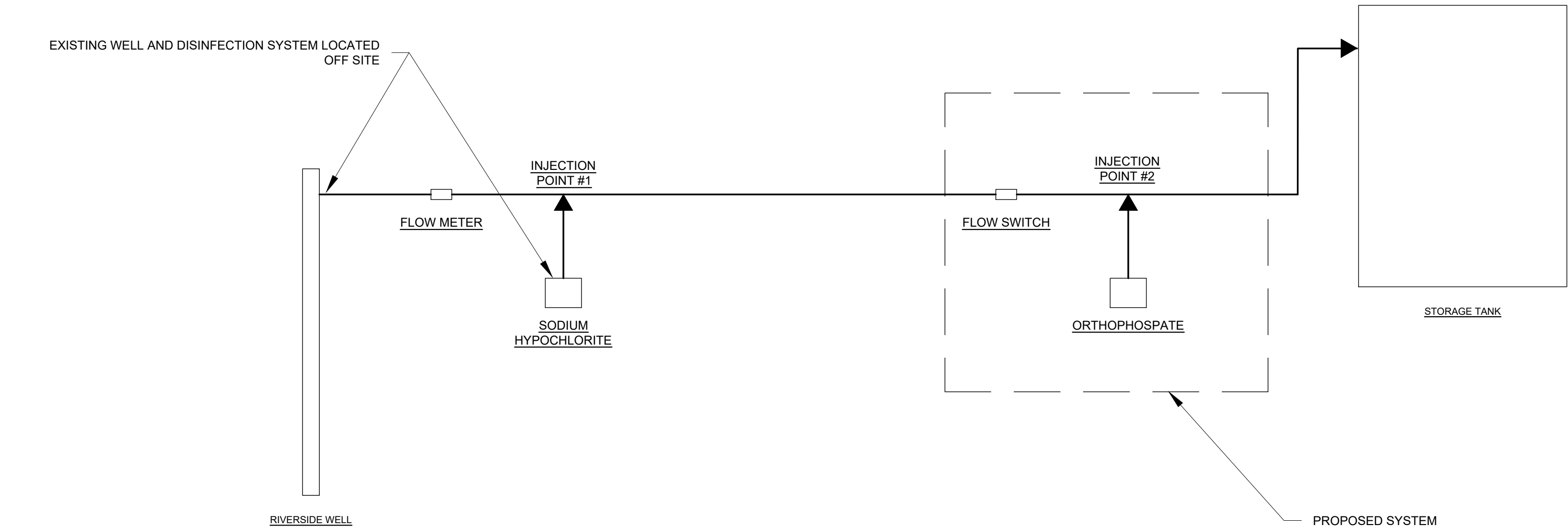
PROCESS FLOW DIAGRAM NOT TO SCALE
