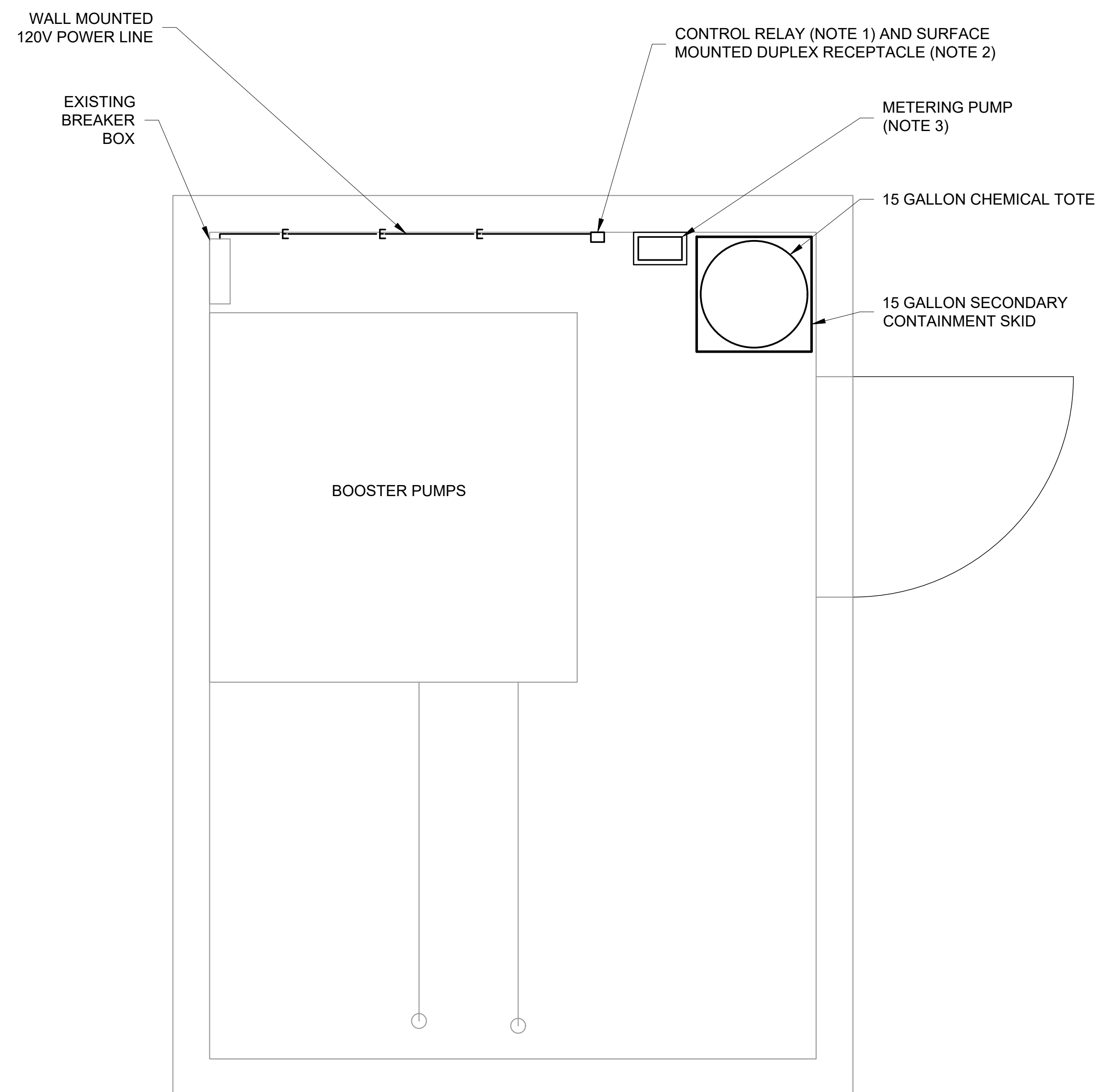
PLAN VIEW
